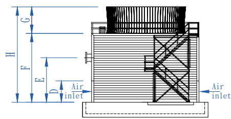
寬邊視圖 TRANSVERSE ELEVATION
